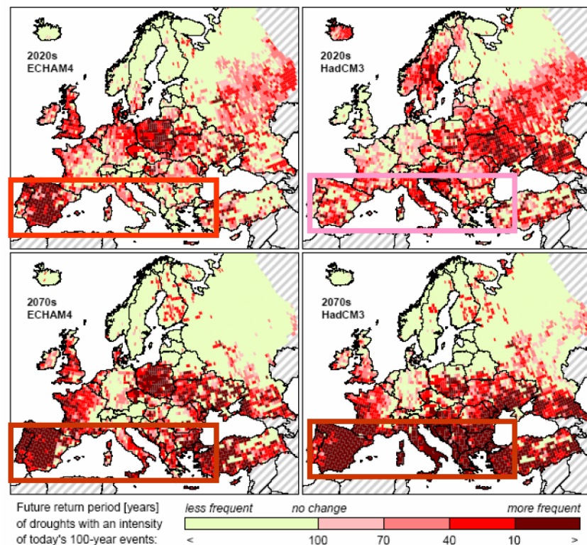
Figure 7: Change in recurrence of 100-year droughts, based on comparisons between climate and water use of 1961-90 and simulations for the 2020s and 2070s (ECHAM4 and HadCM3 climate models, emissions scenario IS92a and a business-as-usual water use scenario). Values calculated with the model WaterGAP 2.1 (Lehner et al., 2005b)
